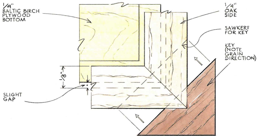
DETAIL: BOTTOM VIEW - Mitered Corner and Key
